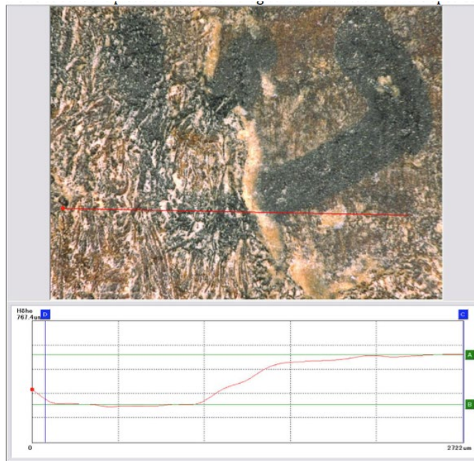
Fig. 2.2. Micrograph and the height measurements performed with a digital microscope.
